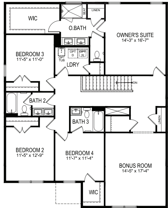
SECOND FLOOR
